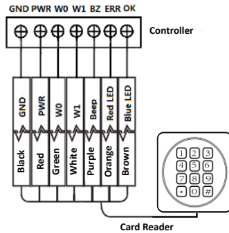
Figure 4-1 Wiring diagram of Wiegand card reader
